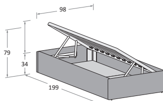
Sfoderabile \ Removable cover
